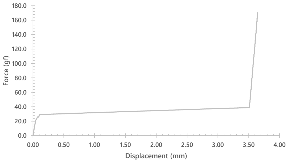
Kailh Aurora Pink (Upstroke)
